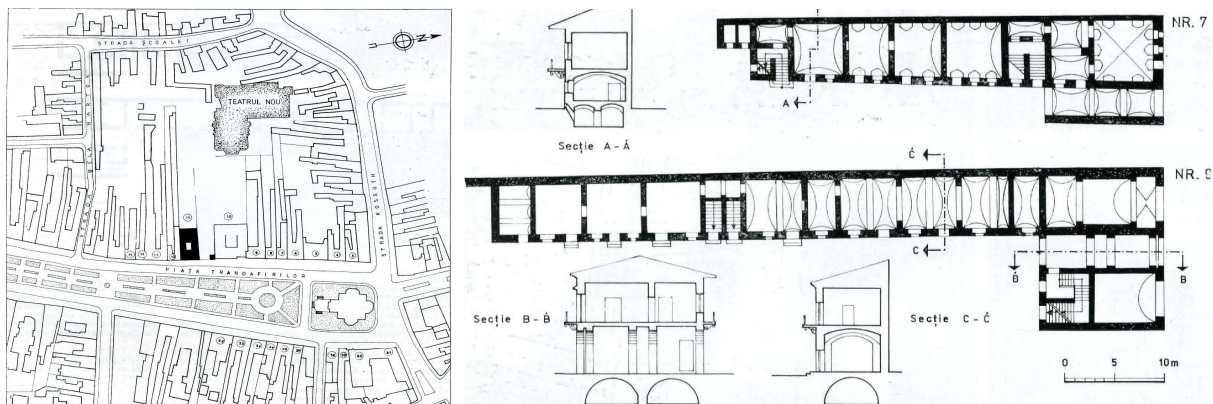
(1) Site plan from 1962 on which the preserved buildings are marked (Toldalagi Palace, respectively the bell tower of the Franciscan Monastery) 22 ; (2) The houses in Piața Trandafirilor no. 7 and 9, demolished in 1971 – Surveys made by D.S.A.P.C. Mr. Mureș, inventory fund D.M.I. 23
